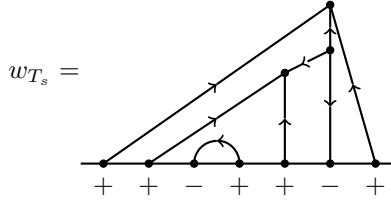
FIGURE 10. The web of content s corresponding to T_s .
