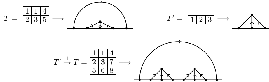
FIGURE 16. Joining two webs.
