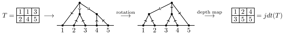
FIGURE 15. Rotation of a web.
