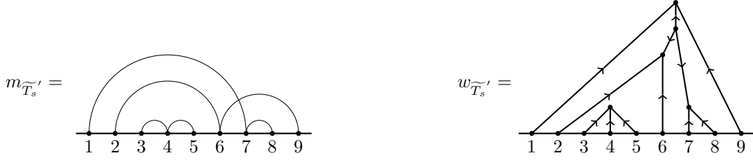
FIGURE 9. The m -diagram and web corresponding to \widetilde{T}_s' .
