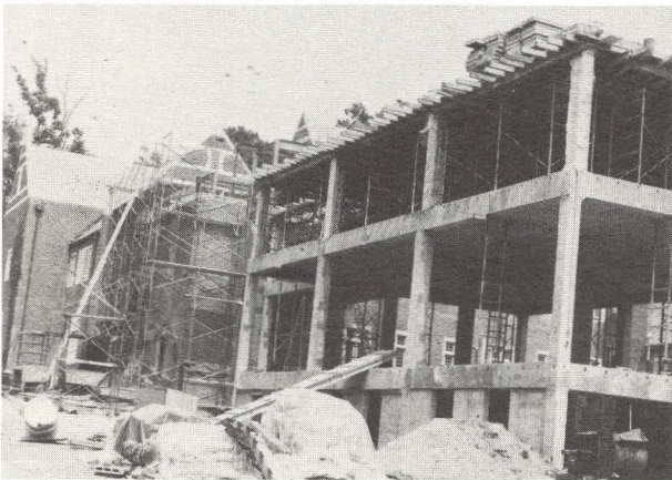
Pouring Third-Floor--Spring-1980
