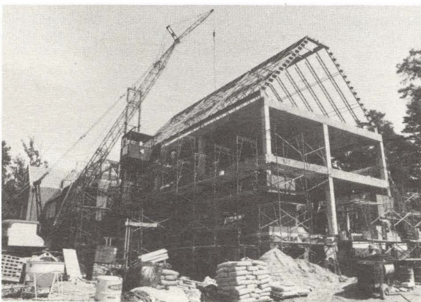
Steelgirders for roof--Summer-1980
