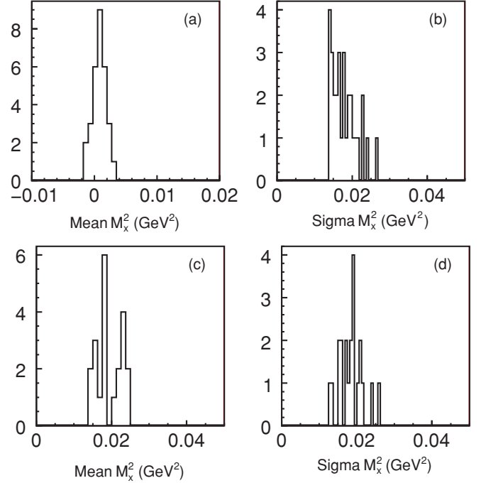
FIG. 15. Distribution of the means and standard deviations of the Gaussian functions for the photon and pion peaks for sub-bins of one kinematical bin: 1.7 < Q^2 < 2.8 (GeV/c) 2 and 0.1 < |t| < 0.8 (GeV/c) 2 .
